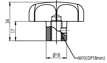
SCSKS316-50
