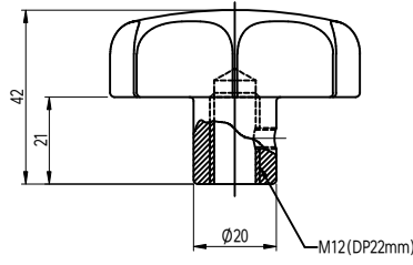
SCSKS316-63
